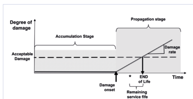
◀ Scheme of the approach for the to-be-developed accelerated test. Flatt R. et al. (2017).
