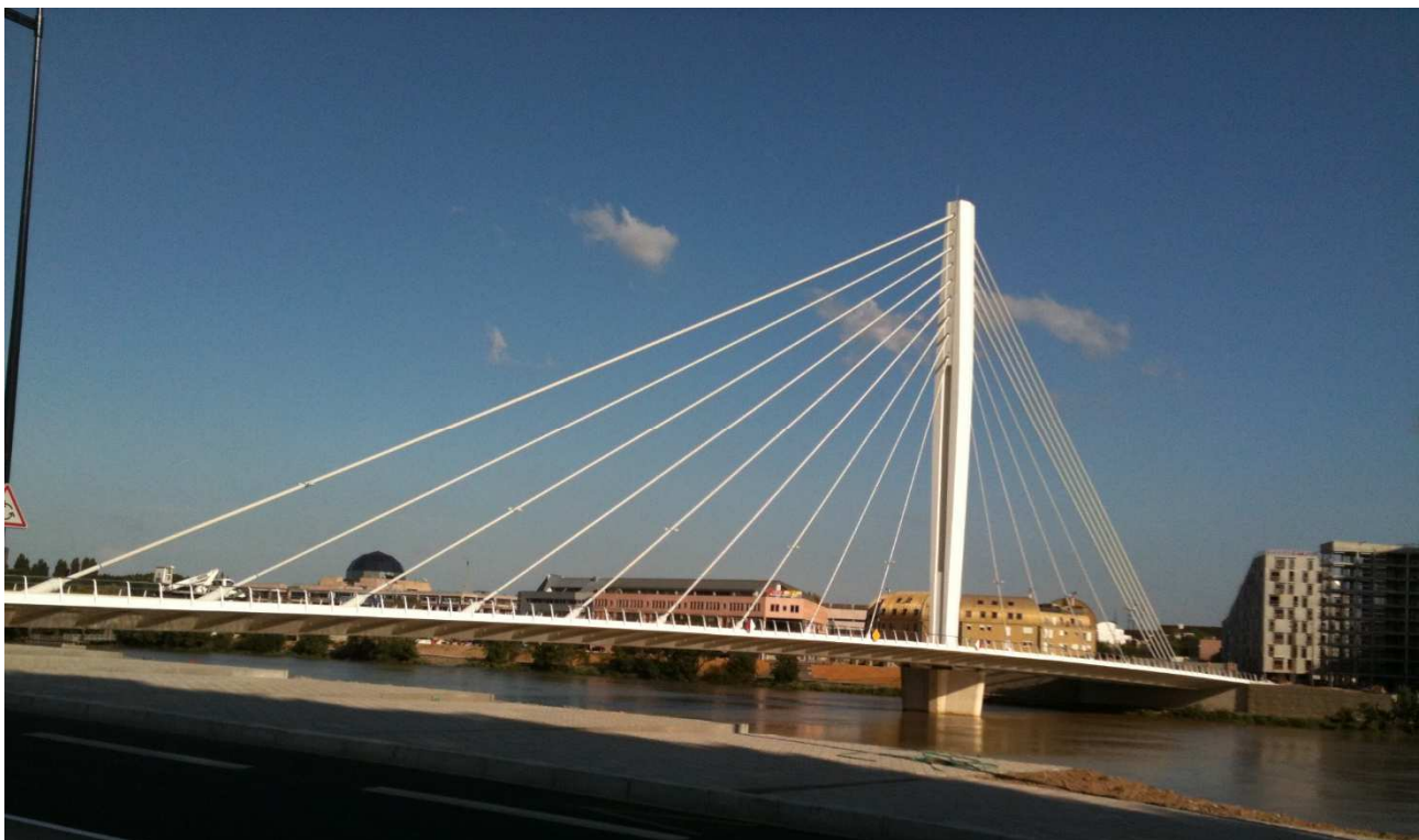
Eric Tabarly Bridge © Michel Royer-Muller
